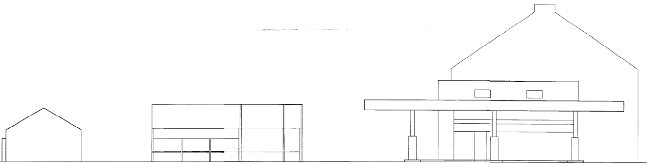
SIDE ELEVATION TO FORECOURT SHOP / CAR WASH & WORKSHOP
